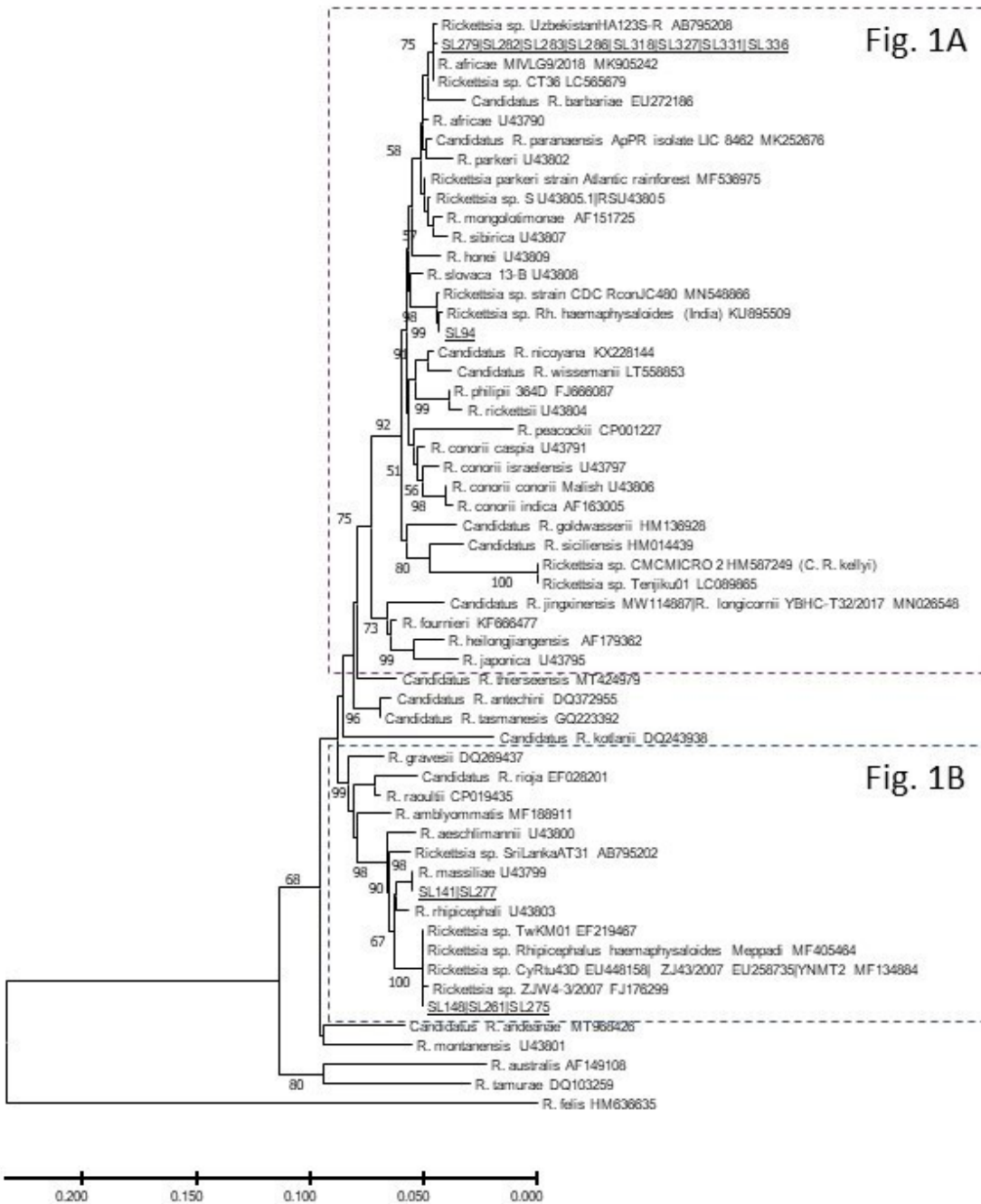
Supplemental Figure 1: OmpA gene fragment genetic relationship of SFG Rickettsia detected in ticks from Sri Lanka. Frames indicated by broken lines correspond to Figure 1A and Figure 1B shown in the main part of the manuscript. Samples of Sri Lankan ticks are indicated by letters SL and corresponding tick number and are underlined.
